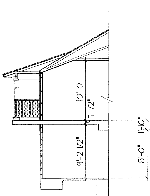
BUILDING SECTION
