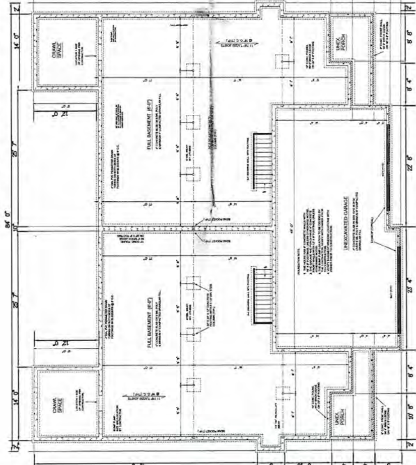
FOUNDATION PLAN
