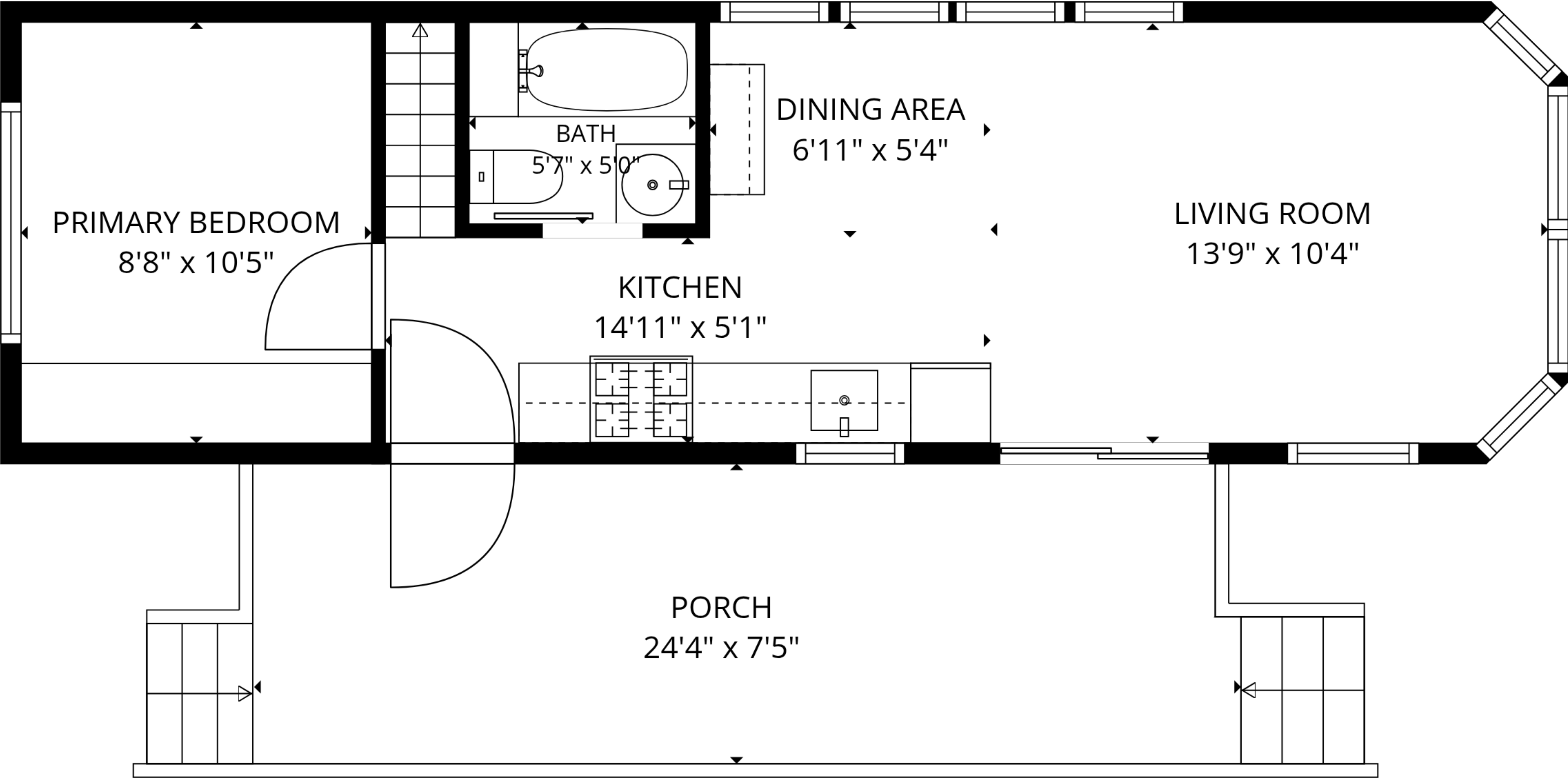
2nd floor
