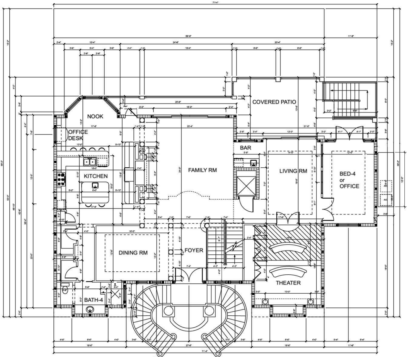
1st FL. DIMENSIONAL FLOOR PLAN
