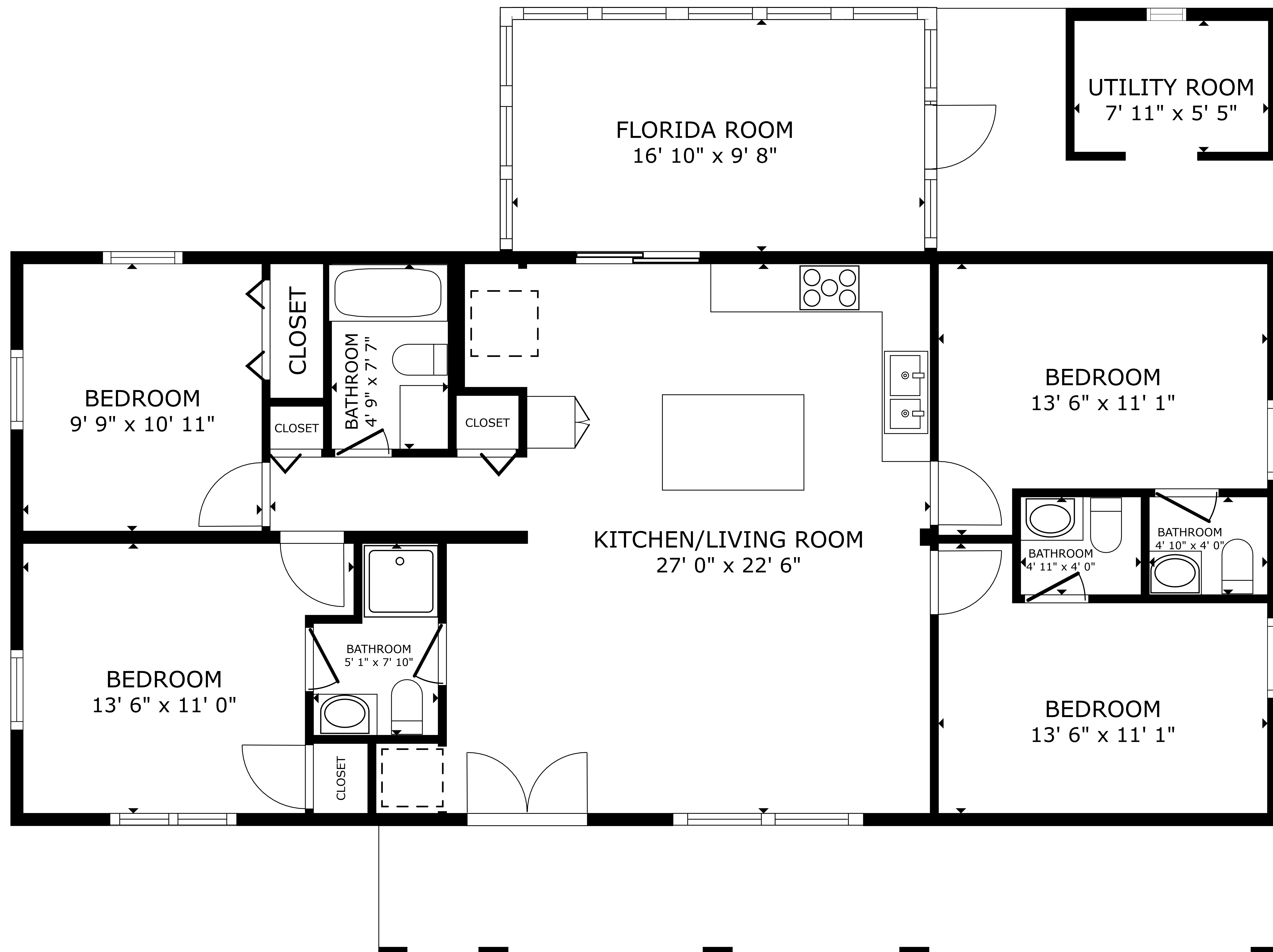
FLOOR PLAN
