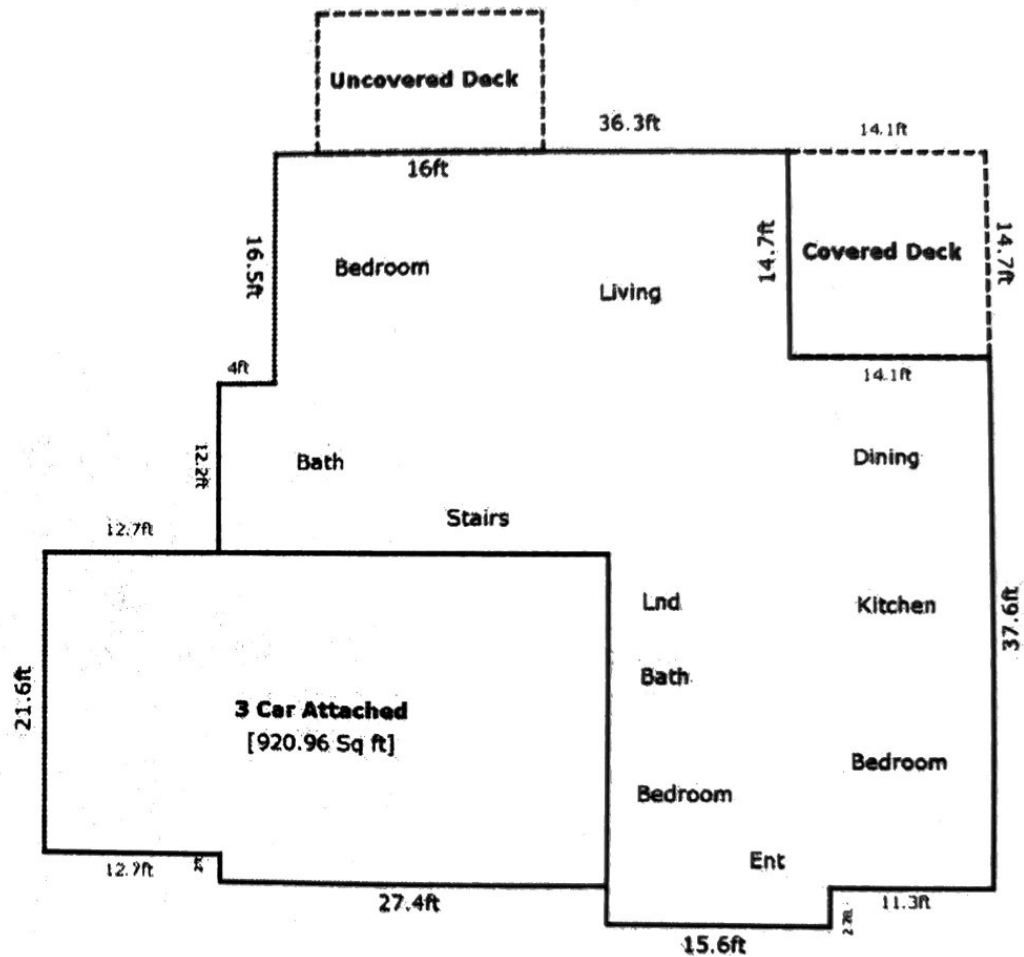
First Floor [1964.97 Sq ft]
