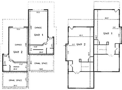
Basement Plan First Floor Plan
